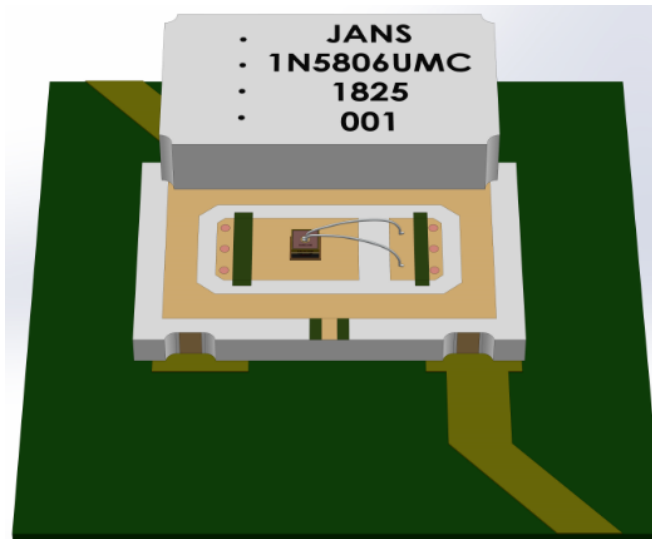
Gold Pads
